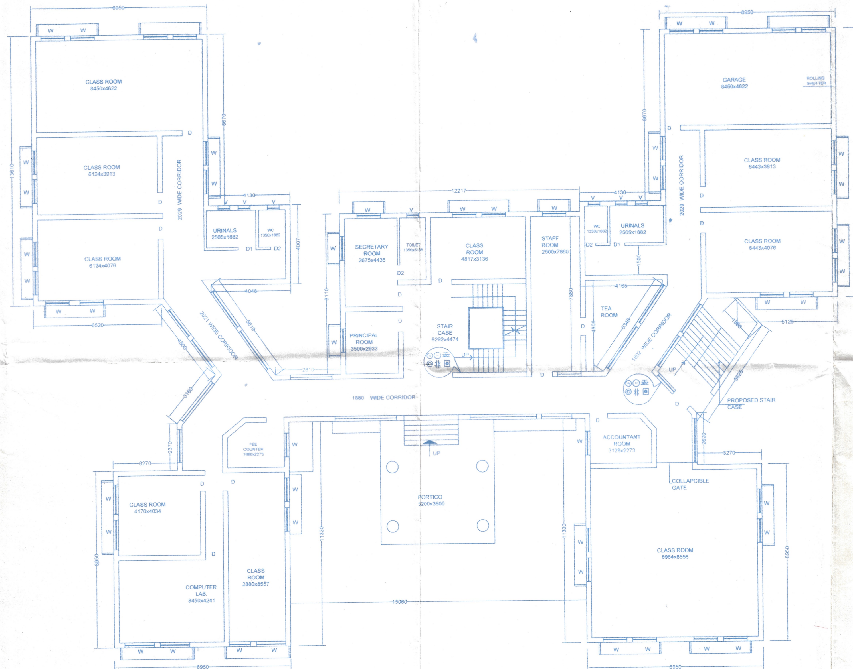
GROUND FLOOR PLAN (EXISTING) AREA=672.60 Sq.m SCALE=1:100
