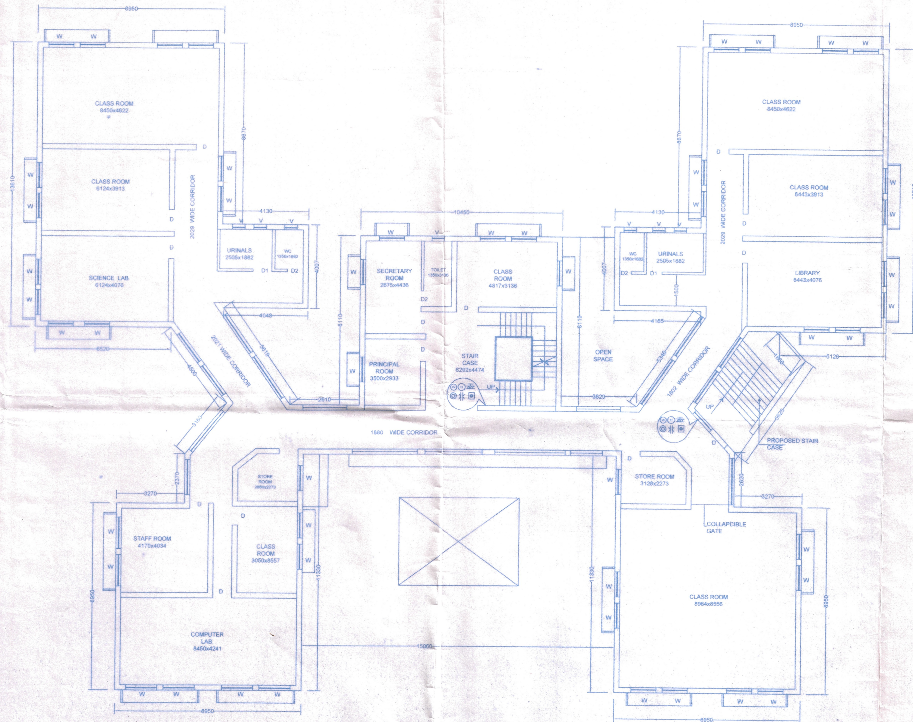
FIRST FLOOR PLAN (EXISTING) AREA=639.82 Sq.m SCALE=1:100
